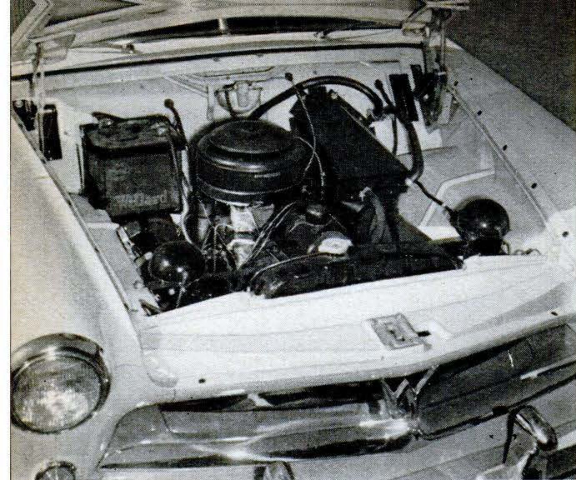
ENGINE has intake manifold cast integrally with block to eliminate gasket that might cause leakage. Cutaway (right) indicates position of single rocker arm for each cylinder, and extra-big intake valve.
